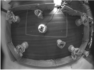
Figure 5: The figure shows phototaxis towards the light source mounted on top of the charging station. A characteristic emergent zig-zag behavior is observed. Notice also the parking behavior which emerges from phototaxis and touch-based obstacle avoidance.
